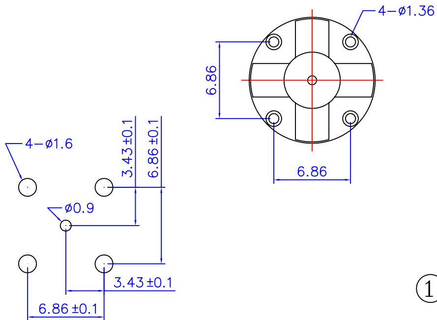
RECOMMENDED PCB BOARD LAYOUT WITHOUT MOUNTING POSTS
