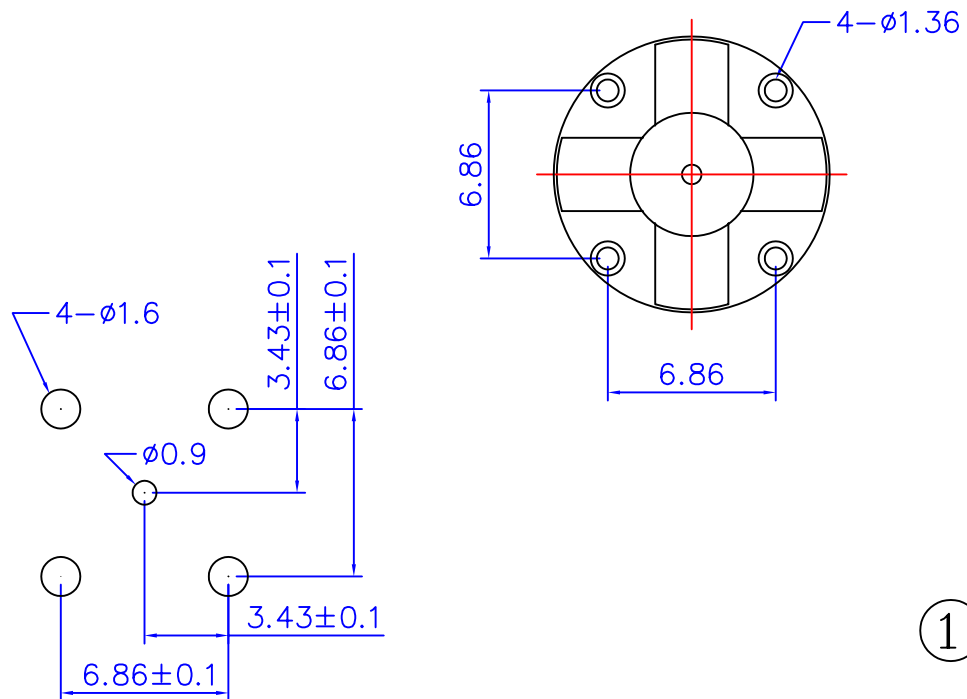
RECOMMENDED PC BOARD LAYOUT WITHOUT MOUNTING POSTS
