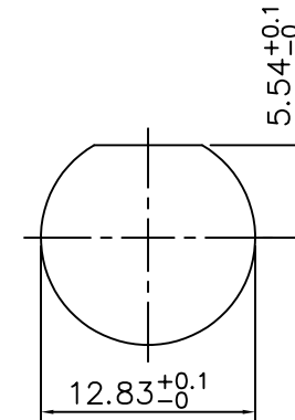
RECOMMENDED MOUNTING HOLE MAXIMUM PANEL THICKNESS: 5.5MM
